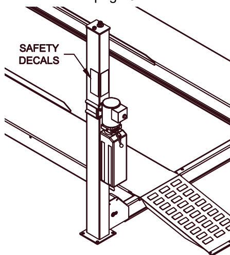
Fig 14 – Safety Decal Placement
